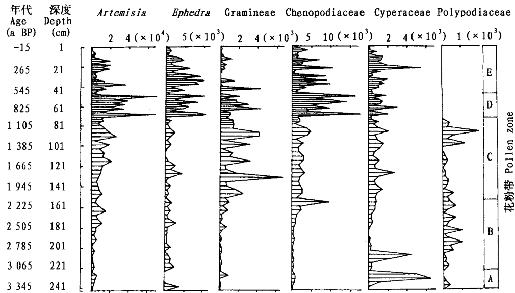
图 4 麦里泥炭剖面化石花粉浓度 (粒/cm 3 ) Fig.4 Pollen concentration for Maili section (grains/cm 3 )
