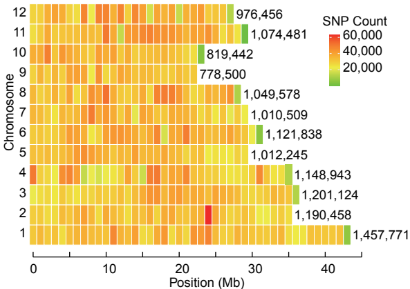
The Number of SNPs within 1Mb Window Size
